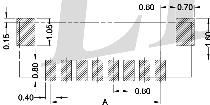
Recommended P.C.B Layout General Tolerance±0.05
