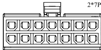
2*7PIN
