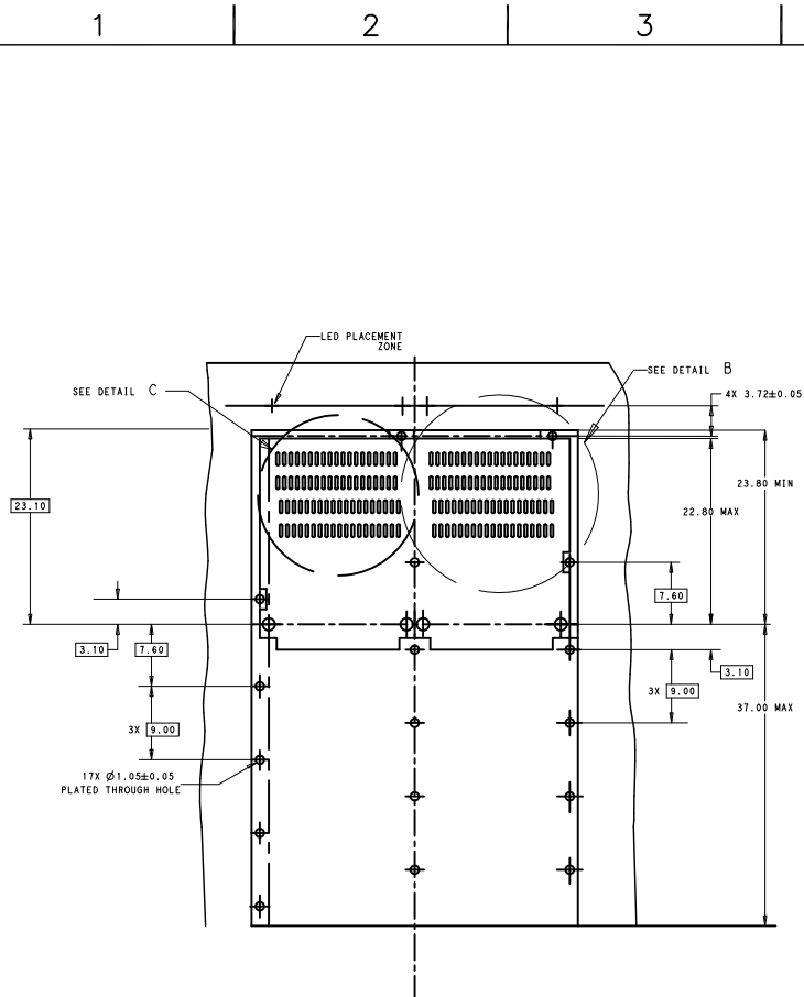
RECOMMENDED SINGLE SIDE MOUNTING PCB BOARD LAYOUT COMPONENT SIDE SHOWN
