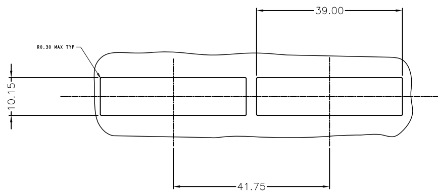
RECOMMENDED PANEL FOR SINGLE SIDE MOUNTING
