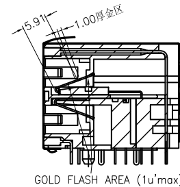
GOLD FLASH AREA (1u"max)
