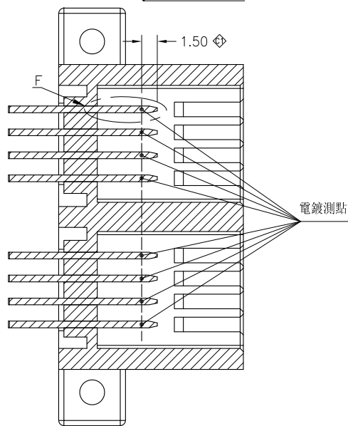
SEC. D-D
