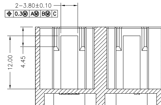
SEC. C-C
