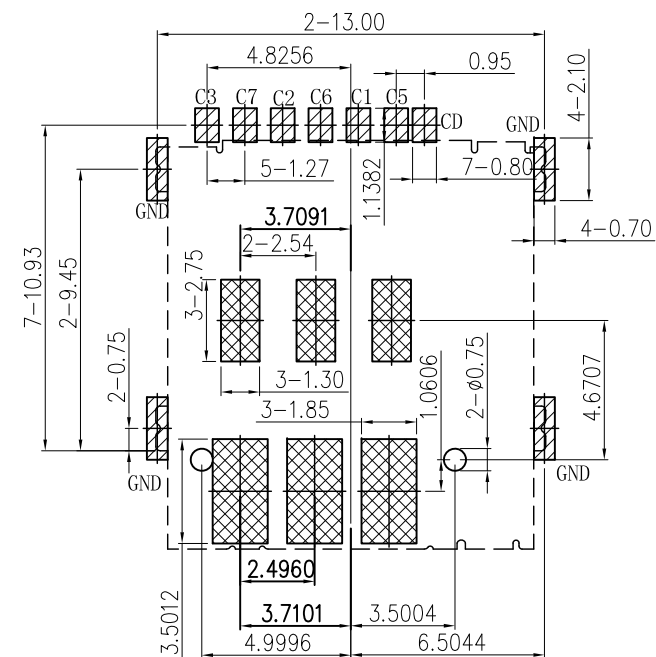
RECOMMENDED PCB LAYOUT TOLERANCE: \pm 0.05
